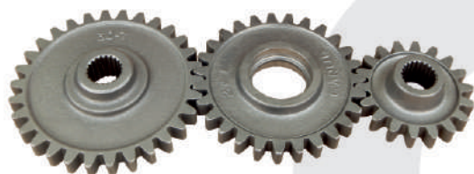
Side Gear Set 30T x 27T x 18T Part No. NR 2748
