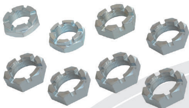
Hex Nut 28 MM | Part No. NR 187 Hex Nut 30 MM | Part No. NR 188 Hex Nut 32 MM | Part No. NR 189 Hex Nut 35 MM | Part No. NR 190 Hex Nut 36 MM | Part No. NR 191 Hex Nut 38 MM | Part No. NR 192 Hex Nut 40 MM | Part No. NR 193 Hex Nut 45 MM | Part No. NR 197
