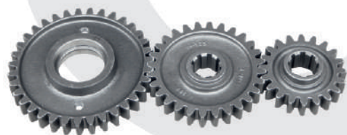
Side Gear Set 35Tx28Tx20T Part No. NR 475
