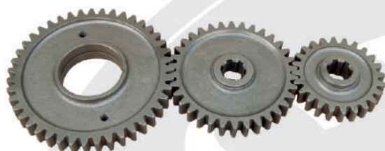
Side Gear 43Tx34Tx24T Part No. NR 2712
