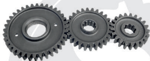
Side Gear Set (36Tx26Tx21T) Part No. NR 1517
