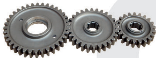
Side Gear Set 36Tx28Tx21T Part No. NR 157
