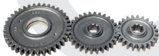
Side Gear Set 37T x 28T x 23T Part No. NR 202
