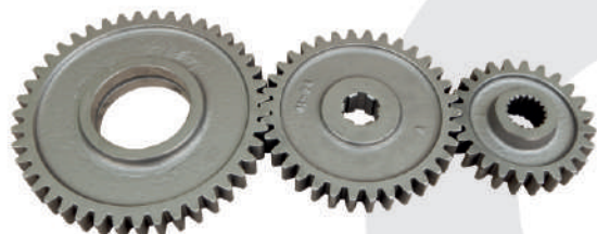
Side Gear 43T x 34T x 24T Part No. NR 2730
