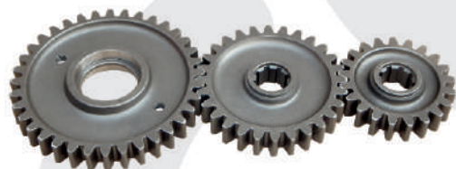
Side Gear Set 36Tx28Tx21T Part No. NR 161
