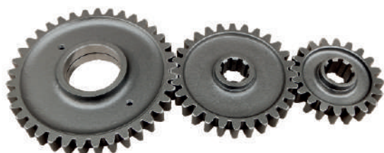
Side Gear K.S. 37T x 28T x 20T Part No. NR 3706
