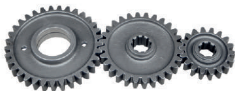
Side Gear Set 33Tx28Tx18T (Inner 8S) Part No. NR 1381
